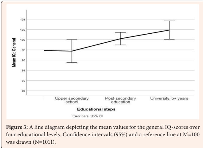
Figure 3: A line diagram depicting the mean values for the general IQ-scores over four educational levels. Confidence intervals (95%) and a reference line at M=100 was drawn (N=1011).
