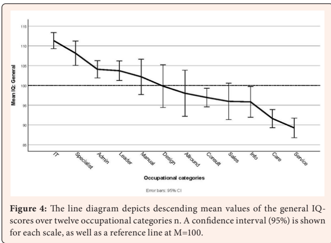
Figure 4: The line diagram depicts descending mean values of the general IQ-scores over twelve occupational categories. A confidence interval (95%) is shown for each scale, as well as a reference line at M=100.
